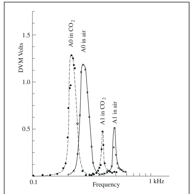
Figure 2. Frequency responses for A0 and A1 in air (crosses) and CO 2 (circles).
