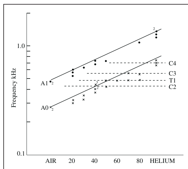
Figure 5. Measured A0 and A1 peak frequencies in air/ He(5N) atmospheres as a function of the He(5N) content in percent. The trend lines show the expected frequency shifts according to Table I. Multiple symbols for certain gas mixtures indicate multiple peaks in the frequency responses. The numbers at some data points refer to identical values obtained in separate runs. The dashed horizontal lines indicate the frequencies of prominent body modes of the violin used in the experiments.
