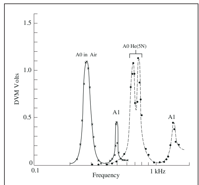
Figure 3. Frequency responses for A0 and A1 in air (crosses) and He(5N) (circles). A doublet is observed for A0 in He(5N).
