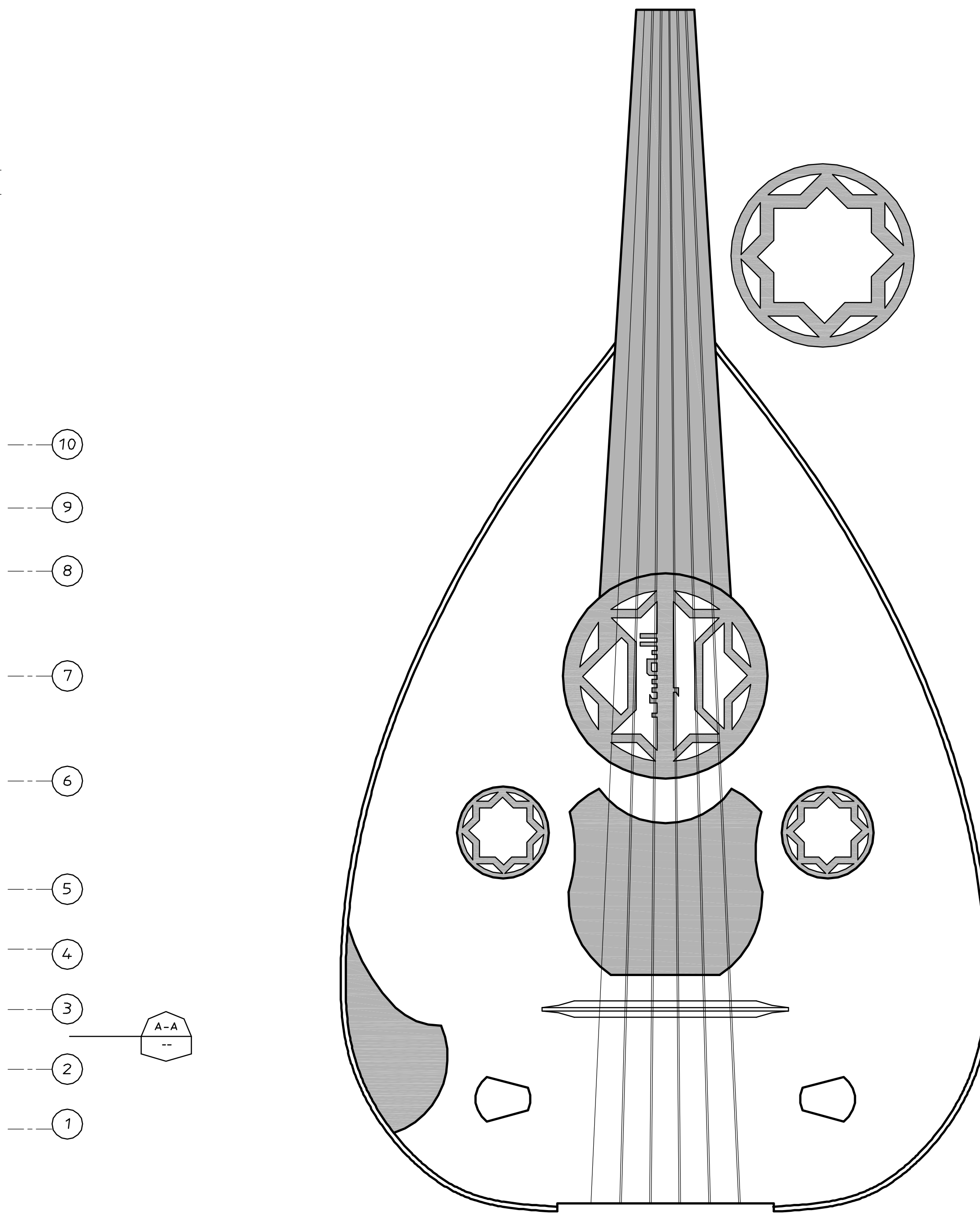
SOUND BOARD FRONT VIEW SCALE 1 / 2
