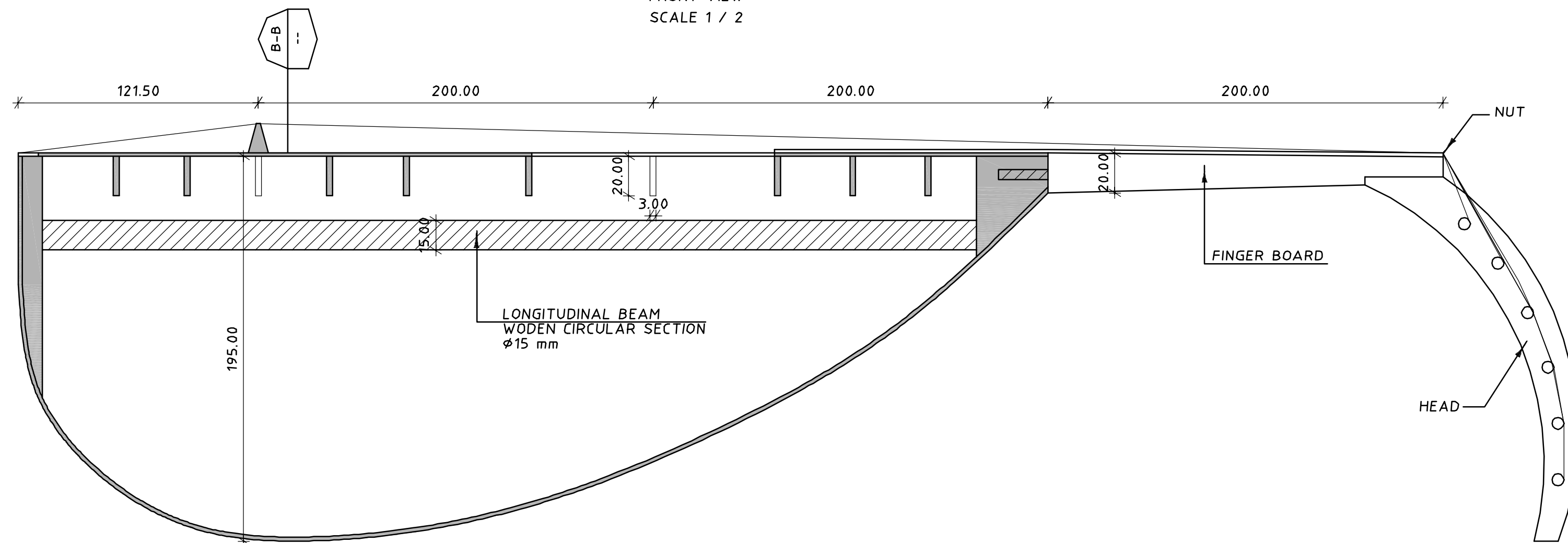
SOUND BOARD FRONT VIEW SCALE 1 / 2
