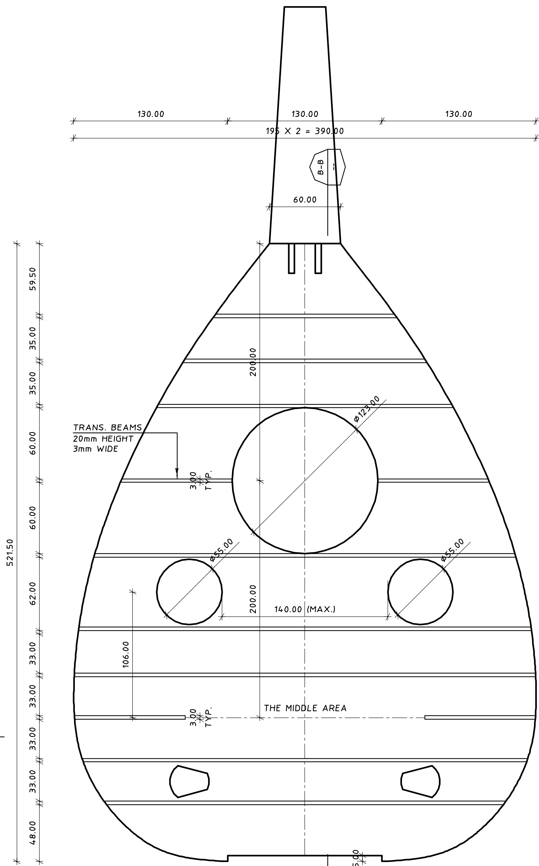
SOUND BOARD TRANSVERSAL BEAM LAYOUT SCALE 1 / 2
